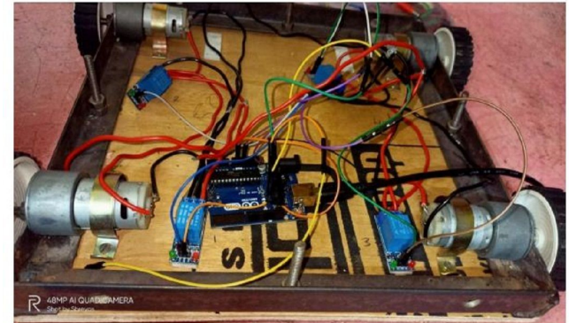
CDR Base with Circuit connections
